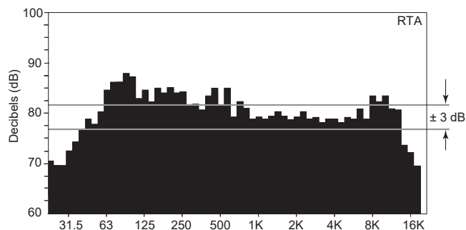
Figure 1: On-axis frequency response in standard stud wall with four coats of latex paint applied to the speaker face panel.
